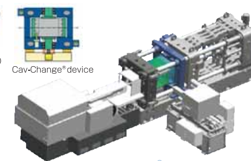
Cav-Change® System
